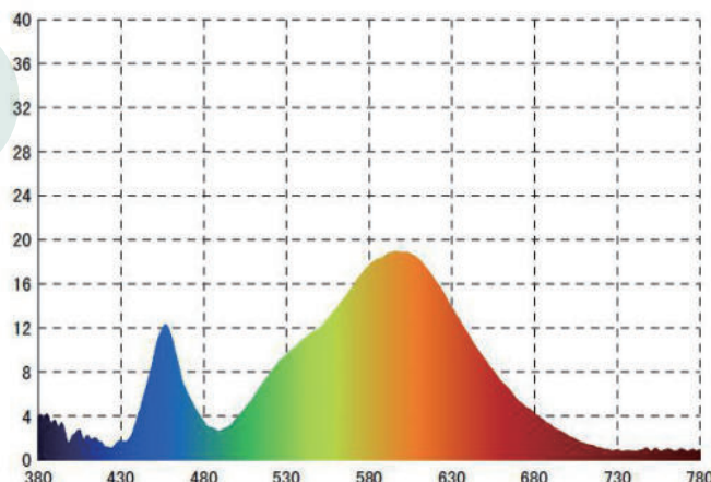
Absolute spectrum
