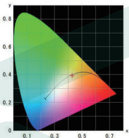
Chromaticity diagram
